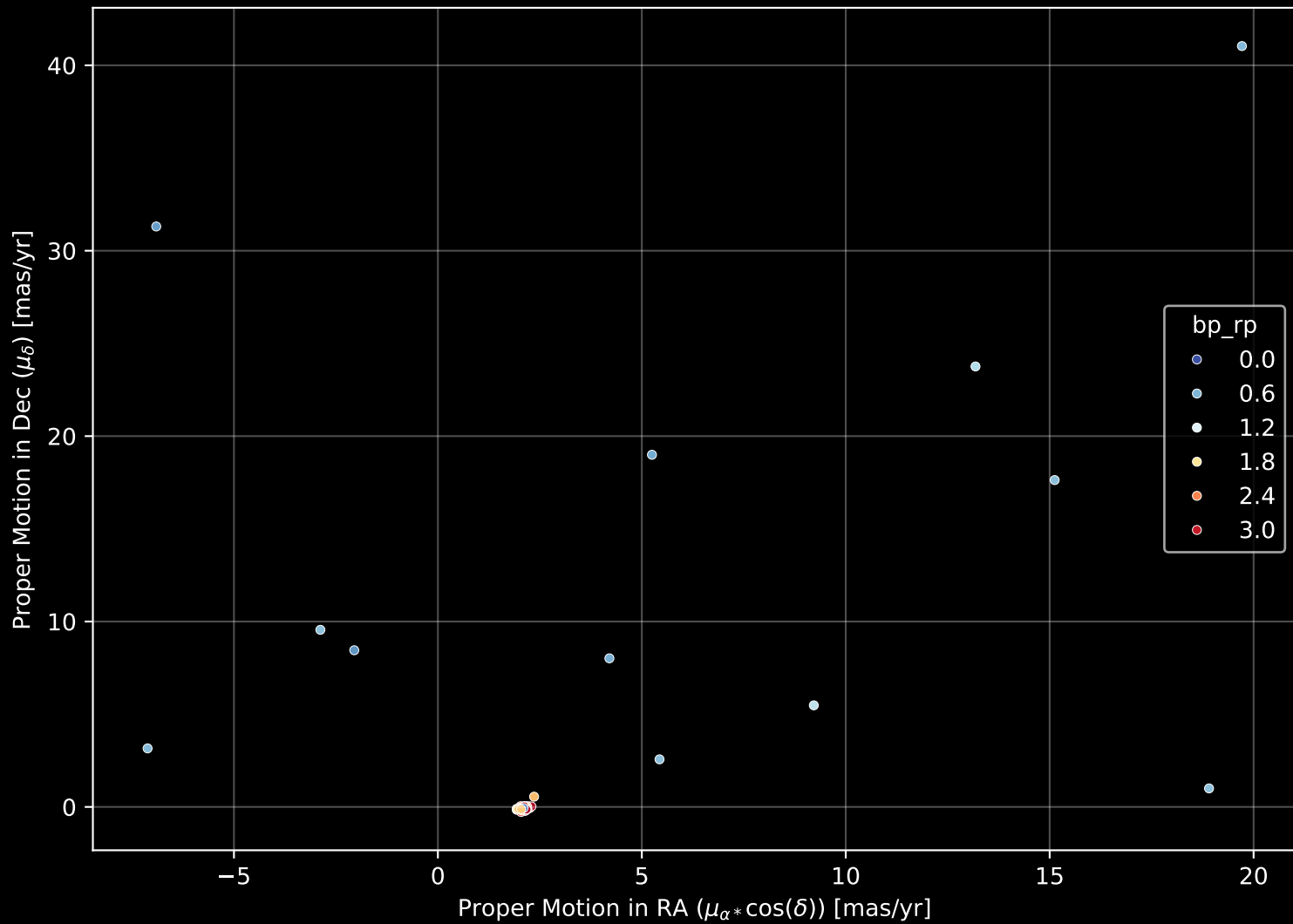
APOGEE DR17 Field: [282-35-O] Proper Motion Diagram (n= 54)
