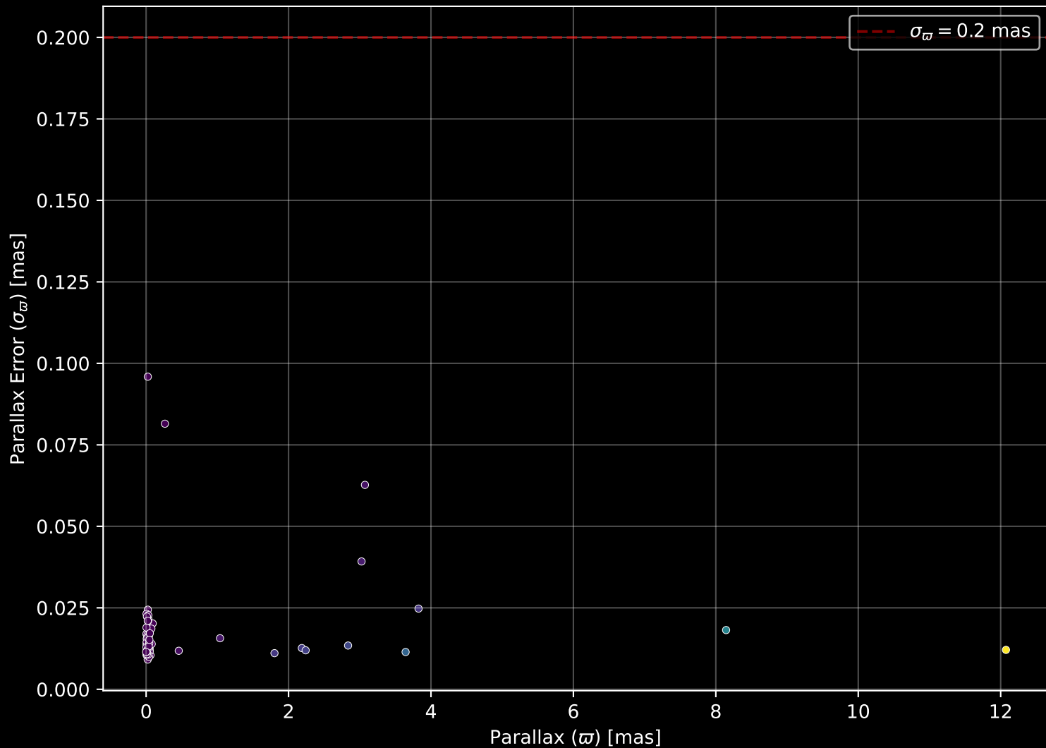
APOGEE DR17 Field: [282-35-O] Parallax Quality (n= 54)
