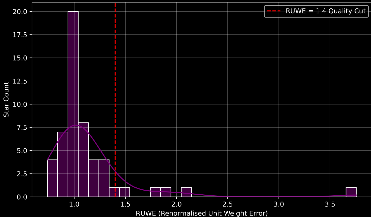
GAPOGEE DR17 Field [282-35-O] RUWE Distribution (n= 53)
