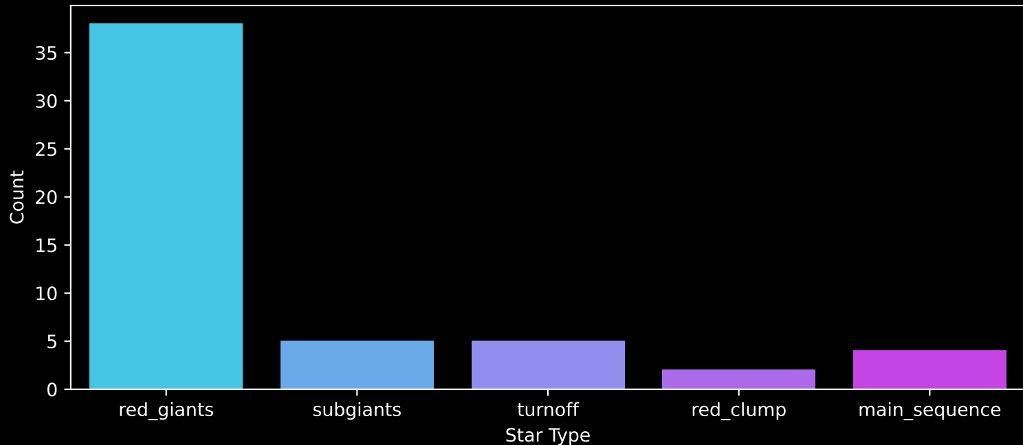
APOGEE DR17 Field: [282-35-O] Count plot of Star Type
