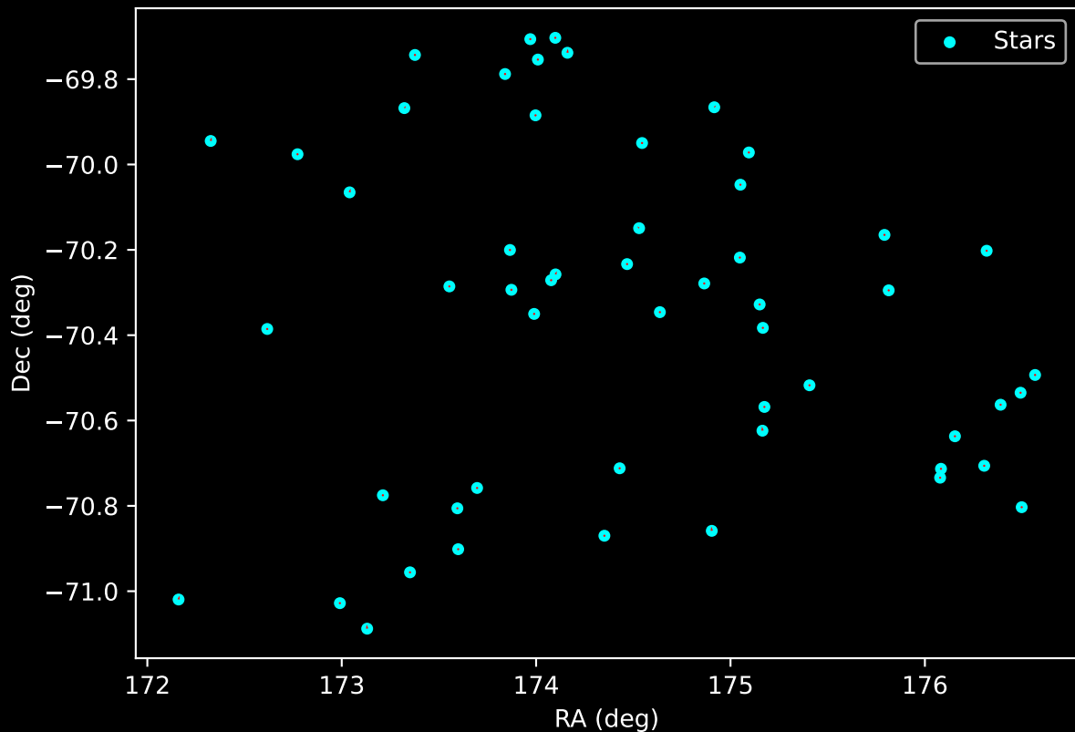
APOGEE DR17 Field: [282-35-O] Proper Motion Vectors for Gaia Star Field (n= 54)
